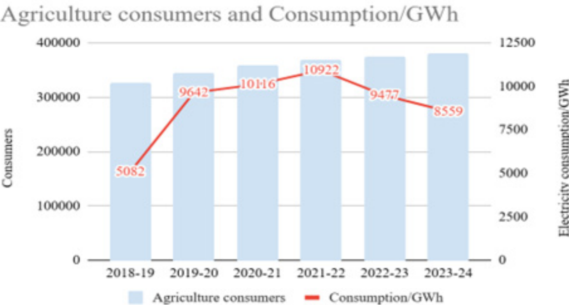
Figure 23 : Electricity Consumption trends agriculture sector
