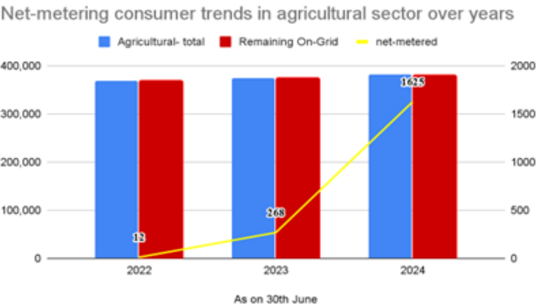
Figure 24 : Net Metering consumers trends across Agricultural sector
